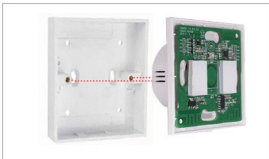
③ Use the screws to fix the back enclosure into the box
